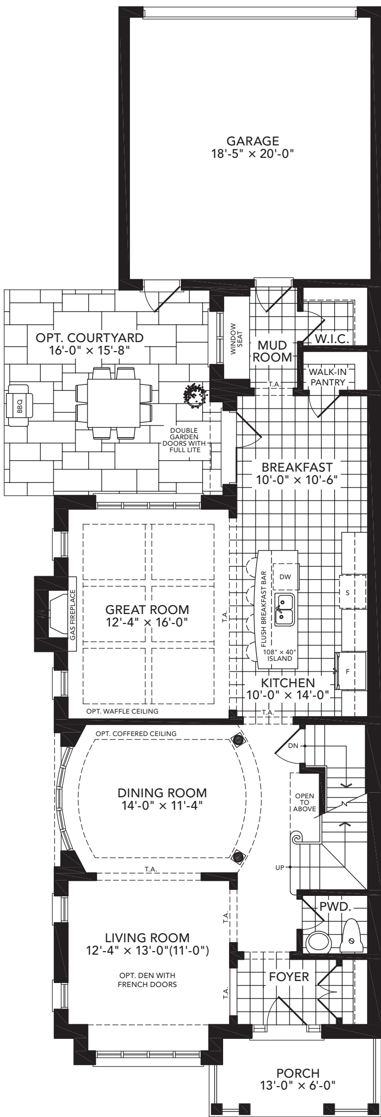
Ground Floor
