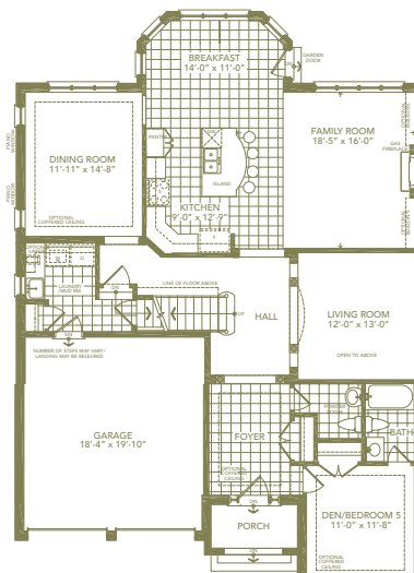
Optional Ground Floor Elev. A
