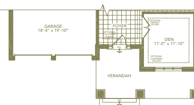
Partial Ground Floor Elev. B
