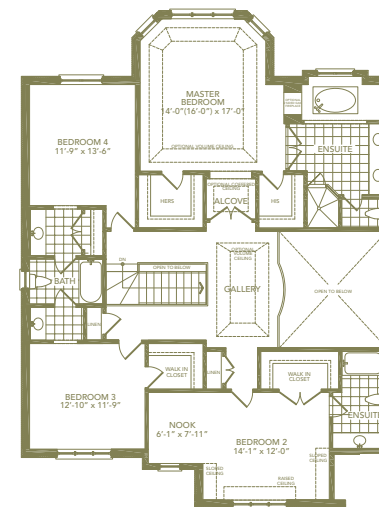
Second Floor Elev. A
